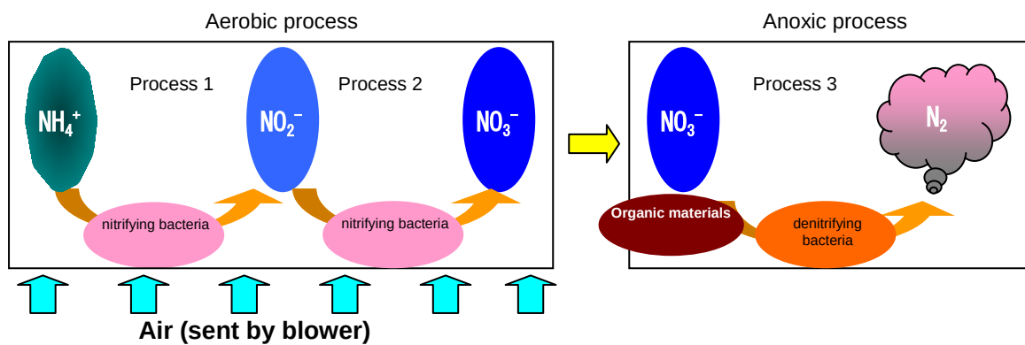
Fig. 3 Conventional treatment (Nitrification-denitrification method)
